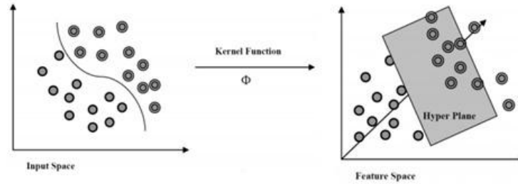
Figure 8: Nonlinear separation using fan kernel SVMs (Borges, 1998)
