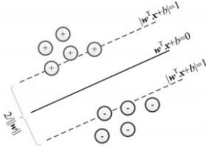
Figure7: A view of binary linear SV (Amin Ghasemi Esfahalan, 2013)
