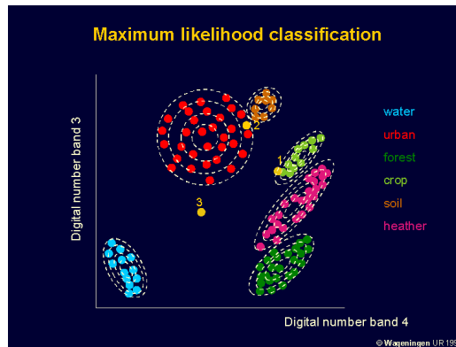
Figure 5: maximum likelihood classification (Alavi Panah, 2013)
