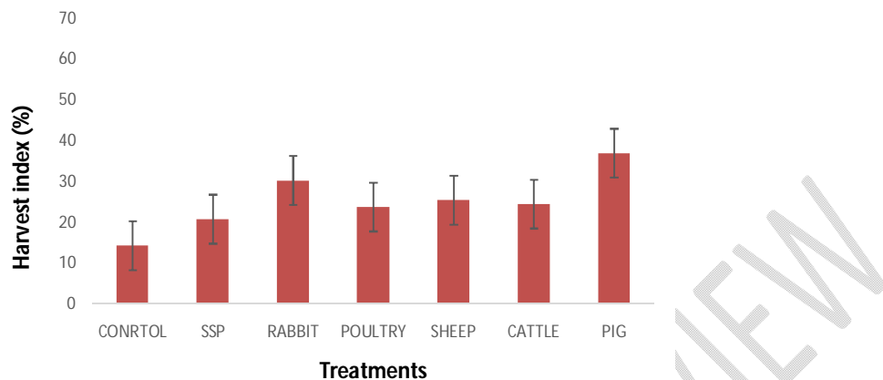
Fig. 2. Effect of treatments on harvest index soybean
