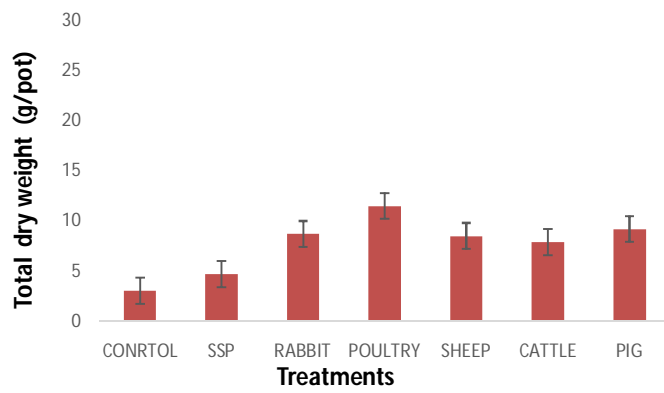
Fig. 1. Effect of treatments on total dry weight of soybean SSP; Single Super Phosphate Bar is standard error of mean
