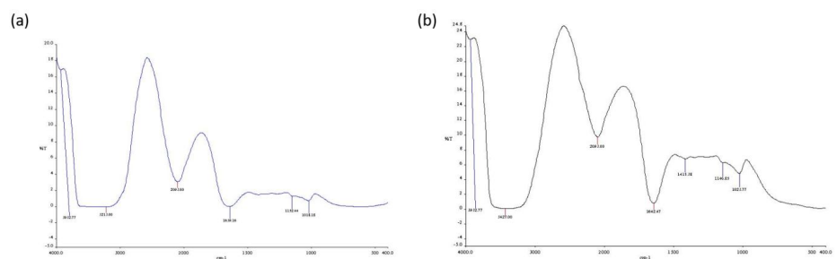
Figure 3: FT-IR spectrum of the exopolysaccharide produced by (a) Leuconostoc mesenteroides (b) Lactiplantibacillus plantarum
