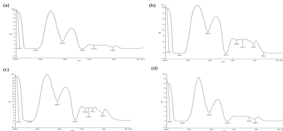
Figure 2: FT-IR spectrum of the exopolysaccharide produced by (a) Lactobacillus delbrueckii (b) Lactobacillus acidophilus (c) Lactiplantibacillus plantarum (d) Lactobacillus crispatus
