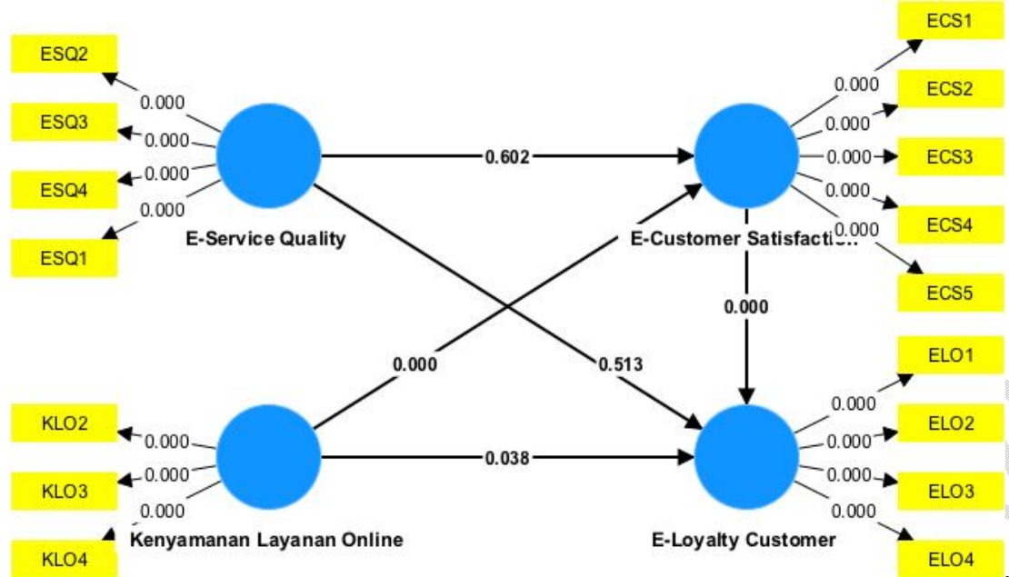
Figure 1 Bootstrapping Procedure
