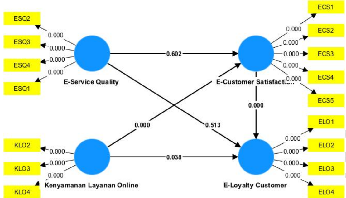
Figure 1.1 Bootstrapping Procedure
