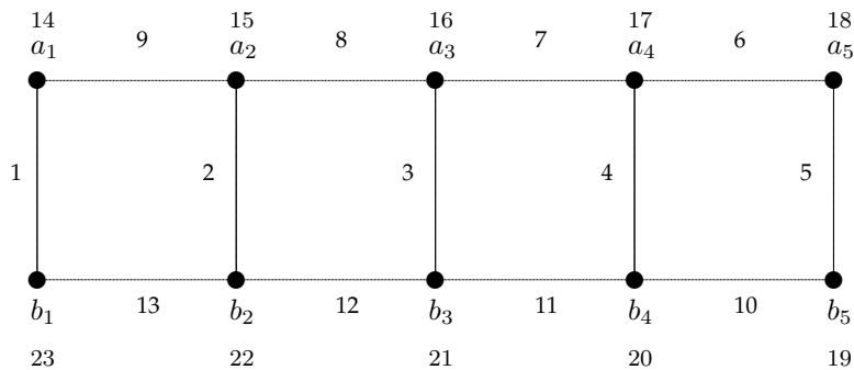
Figure 2 : C_4 - E -SMGL of L_5
