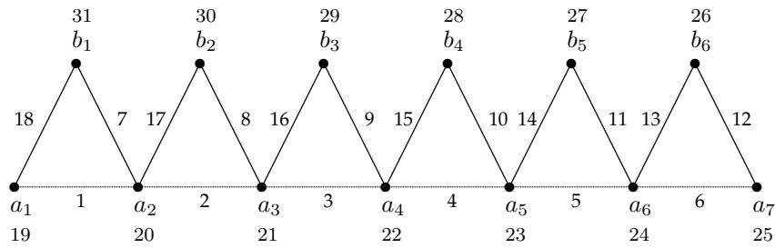
Figure 4: C_3 - E -SMGL of triangular snake \Delta_6
