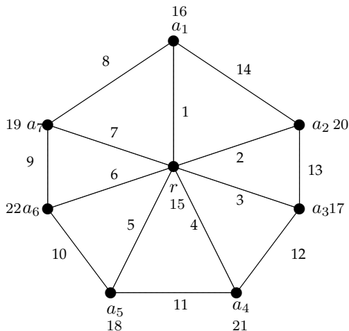
Figure 1 : C_3 - E -SMGL of W_7
