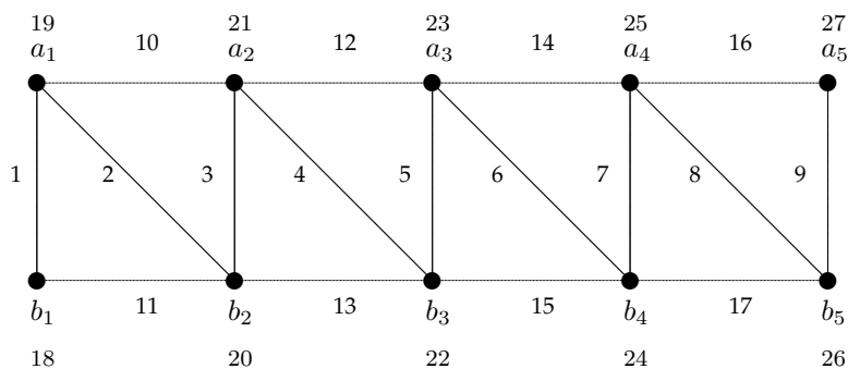
Figure 3 : C_3 - E -SMGL of triangular ladder TL_5
