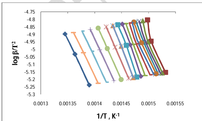
Fig 9: \ln(\beta/T_\alpha^2) vs 1/T_\alpha plots
