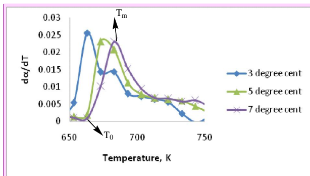
Fig.6: Derivative curves of lanthanum oxalate decomposition at different rates of heating
