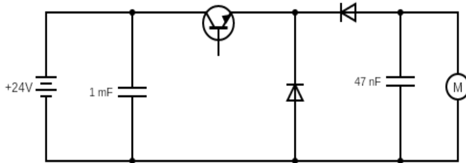
Figure-2: Circuit Diagram of the DC-DC converter
