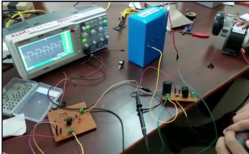
Figure-11: PWM signal at zero acceleration
