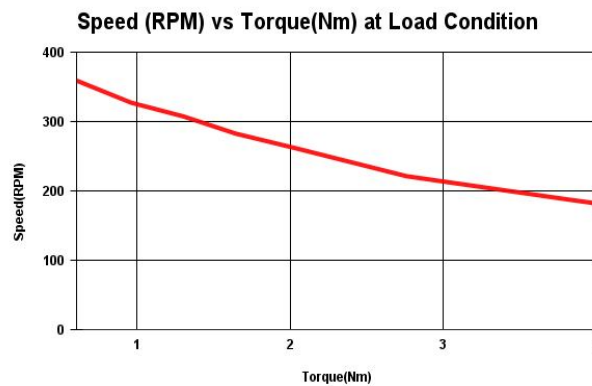
Figure-14: EV Motor Speed-Torque characteristics under Load Conditions
