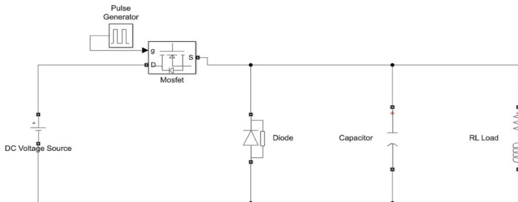
Figure-4: MATLAB/Simulink Circuit Diagram of the converter
