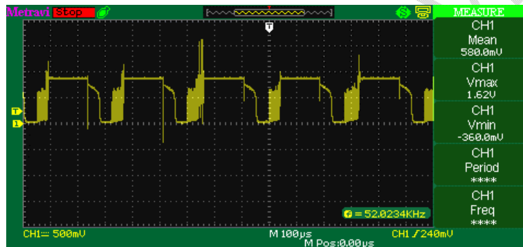
Figure-11: PWM signal at zero acceleration
