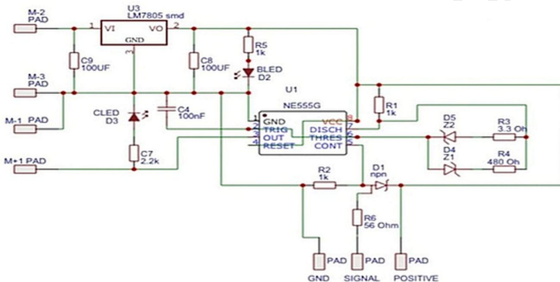
Figure-2: Circuit Diagram of the DC-DC converter
