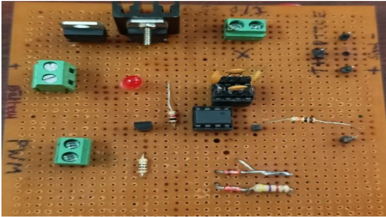
Figure-9: Gate Driver Circuit
