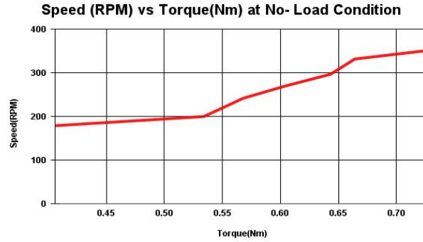
Figure-13: EV motor Speed-Torque characteristics under No-load conditions
