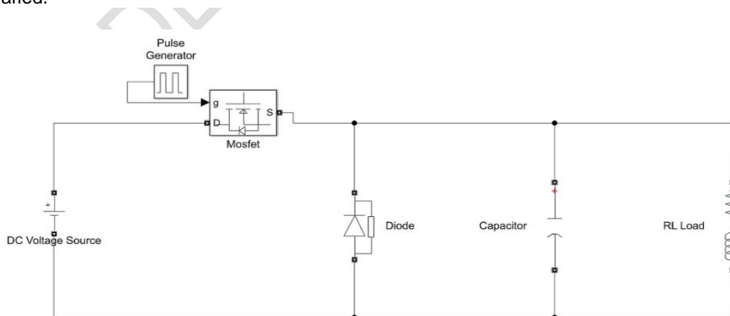
Figure-4: MATLAB/Simulink Circuit Diagram of the converter
