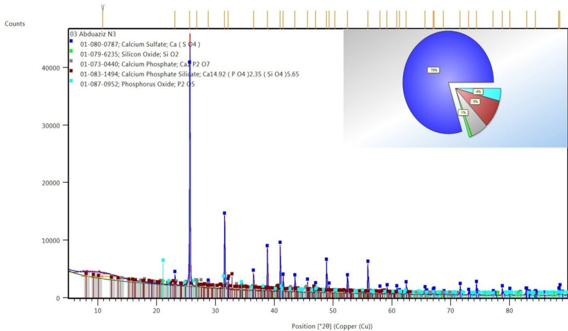
Figure 1. X-ray analysis of a phosphogypsum sample taken, when washed in hot water without mixing in the ratio \text{OPP}:\text{H}_2\text{O}=1,0:2,5 and its salt content.
