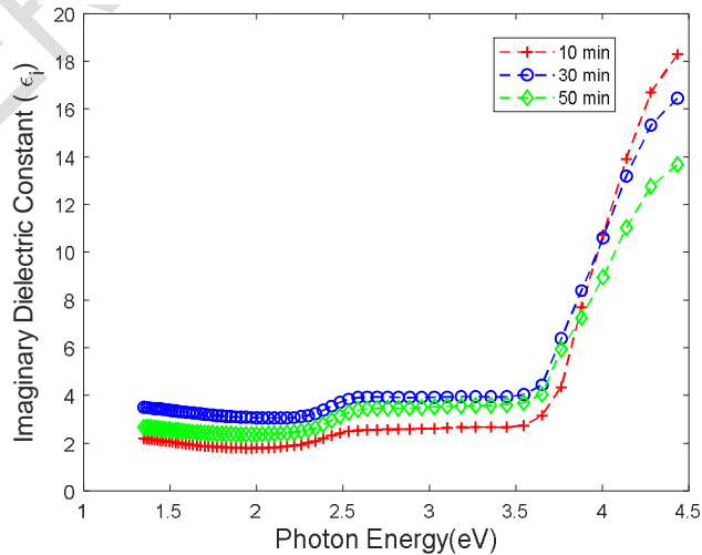
Fig. 7. Plot of Imaginary Dielectric Constant ( \epsilon_i ) vs Photon energy (eV) of CdS thin film of different
