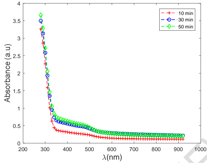
Fig. 2. Variation of absorbance with the wavelength
