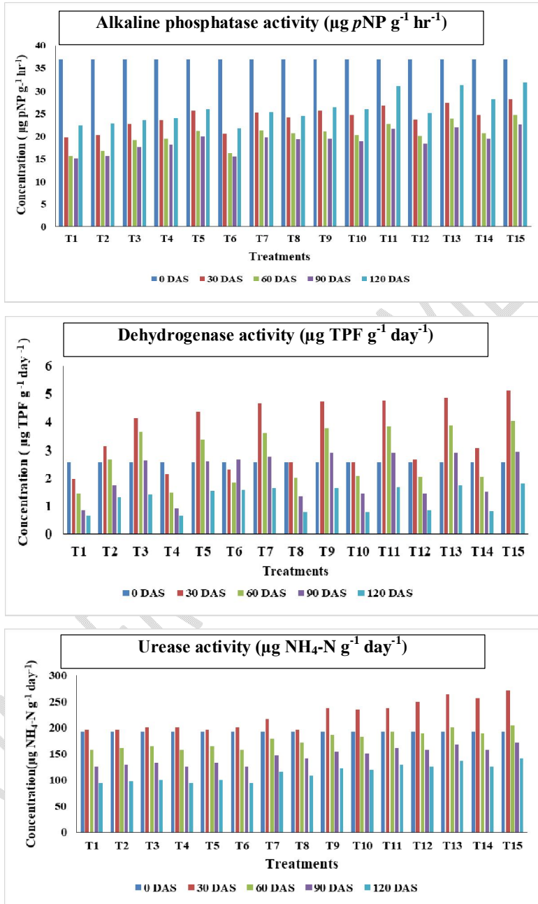
Fig. 2. Enzymatic activities under incubation studies
