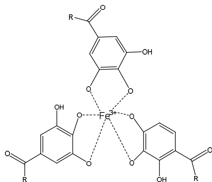
Fig 3: \text{Fe}^{3+} -Tannic acid complex
