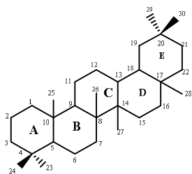
Fig 4: pentacyclic triterpenoid
