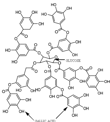
Fig 2: Tannic acid
