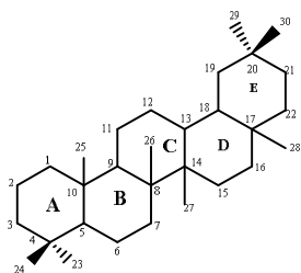
pentacyclic triterpenoid
