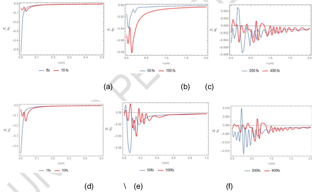
Fig.2. (a) The potential at \pi/6 for t = 1, 10 fs , (b) The potential at \pi/6 for t = 50, 100 fs , (c)
