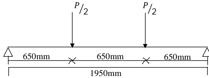
Figure 7: Beam loaded equally at the third points.
