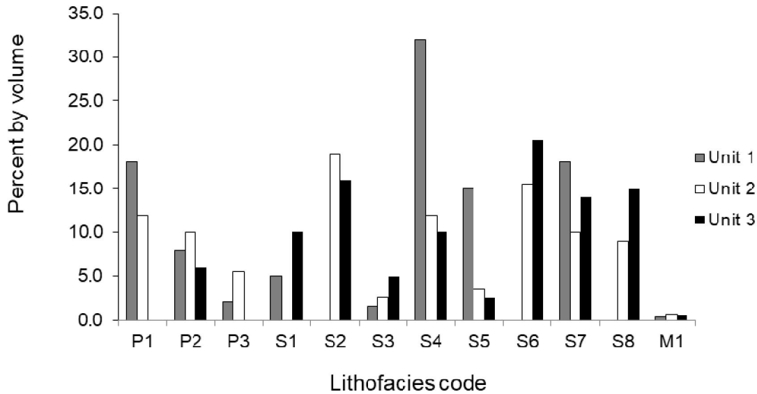
Figure 8. Comparative lithofacies composition of Unit 1, Unit 2, and Unit 3 sandstones in the braidplain sandstone body.
