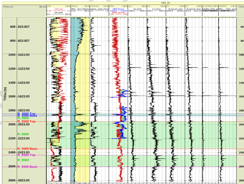
Figure 5: Elastic rock properties estimated for HAX 01
