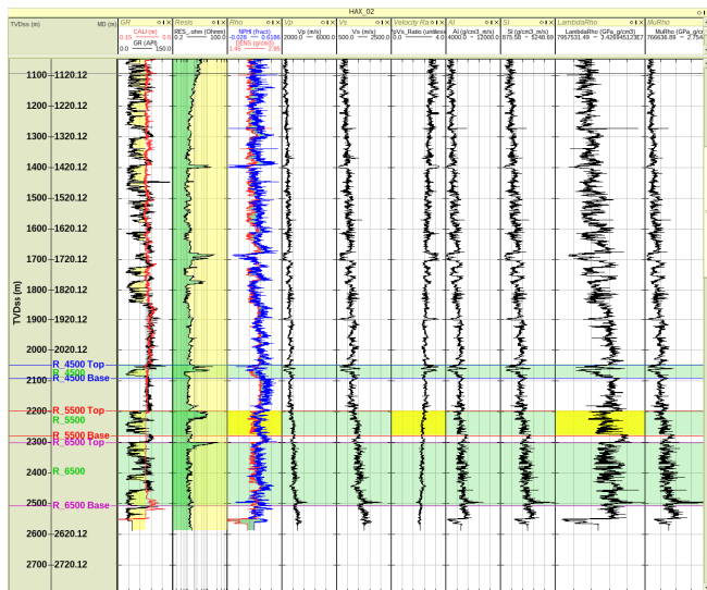
Figure 6: Elastic rock properties estimated for HAX 02
