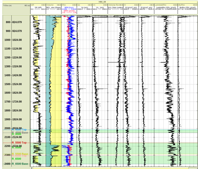
Figure 8: Elastic rock properties estimated for HAX 04
