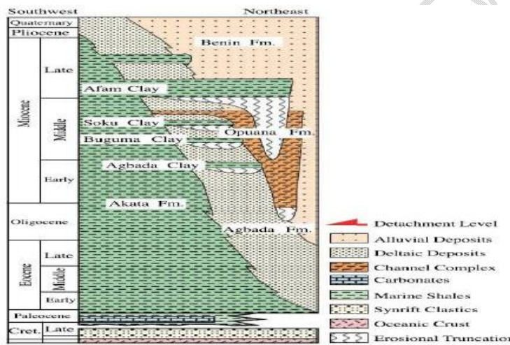
Figure 2. Regional Stratigraphy of the Niger Delta [25.26].
