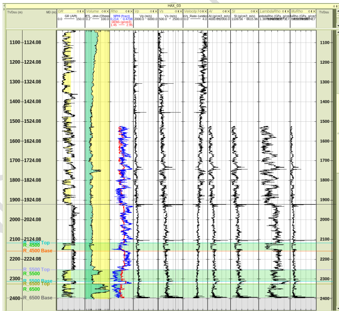
Figure 7: Elastic rock properties estimated for HAX 03
