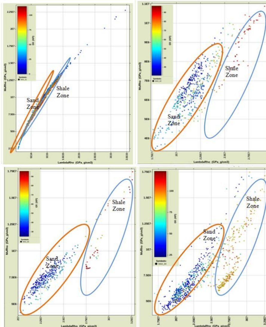
Figure 19: Cross plot of Lambda-Rho ( \lambda\rho ) against Mu-Rho ( \mu\rho ) color coded with Gamma Ray for (a) HAX 01 (b) HAX 02 (c) HAX 03 (d) HAX 04
