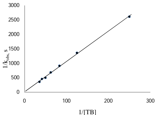
Figure 4: Michealis–Mentens plot of 1/k_{\text{obs}} versus 1/[TB] at [\text{MnO}_4^-] = 2.0 \times 10^{-4} \text{ mol dm}^{-3} , [\text{TB}] = 4.0 \times 10^{-3} - 2.8 \times 10^{-2} \text{ mol dm}^{-3} , I = 1.0 \text{ mol dm}^{-3} (\text{Na}_2\text{SO}_4) and T = 24 \pm 0.1^\circ\text{C} .
