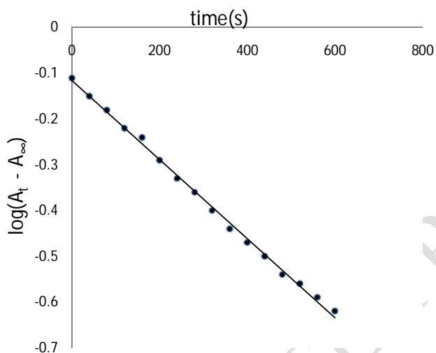
Figure 1: Typical pseudo-first order plot for the redox reaction of TB with MnO_4^- , [TB] = 1.0 \times 10^{-2} \text{ mol dm}^{-3} , [MnO_4^-] = 2.0 \times 10^{-4} \text{ mol dm}^{-3} , [H^+] = 1.0 \times 10^{-2} \text{ mol dm}^{-3} , I = 0.5 \text{ mol dm}^{-3} , \lambda_{max} = 530\text{nm} and T = 23.0 \pm 0.1^\circ\text{C} .
