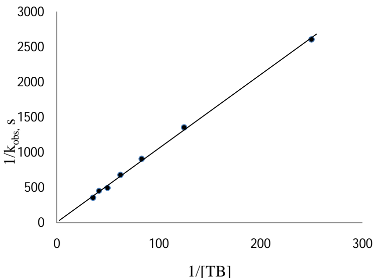
Figure 4: Michealis–Mentens plot of 1/k_{\text{obs}} versus 1/[TB] at [\text{MnO}_4^-] = 2.0 \times 10^{-4} \text{ mol dm}^{-3} , [TB] = 4.0 \times 10^{-3} - 2.8 \times 10^{-2} \text{ mol dm}^{-3} , I = 1.0 \text{ mol dm}^{-3} ( \text{Na}_2\text{SO}_4 ) and T = 24 \pm 0.1^\circ\text{C} .
