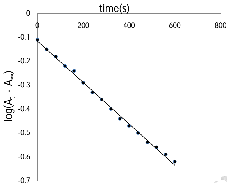
Figure 1: Typical pseudo-first order plot for the redox reaction of TB with MnO 4 - , [TB] = 1.0 × 10 -2 mol dm -3 , [MnO 4 - ] = 2.0 × 10 -4 mol dm -3 , [H + ] = 1.0 × 10 -2 mol dm -3 , I = 0.5 mol dm -3 , λ max = 530nm and T = 23.0 ± 0.1°C.
