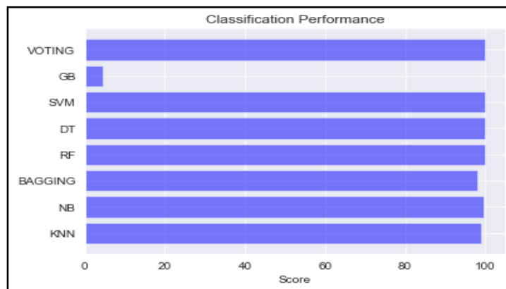
Fig.2: a comparative analysis of Different classification algorithms
