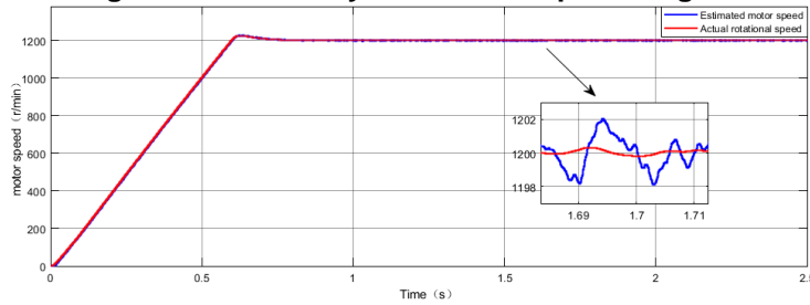
Fig. 5. Speed diagram of improved synovial motor
