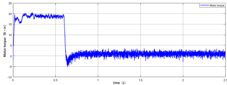
Fig. 8. Traditional synovial torque diagram
