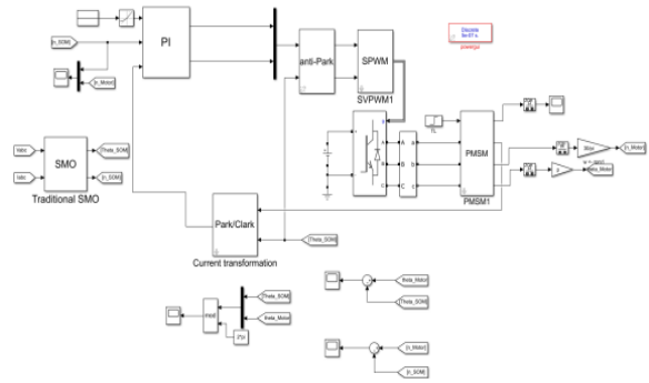
Fig. 3. Simulation model
