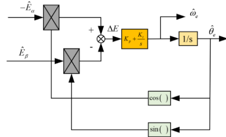
Fig. 1. Traditional PLL structure
