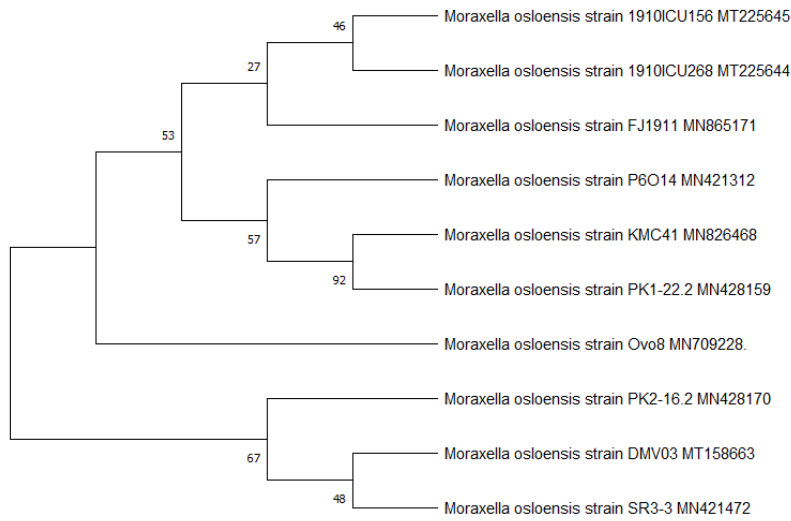
Fig. 3. Phylogenetic tree of Moraxella osloensis DMV03 (MT158663)
