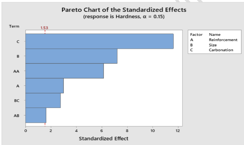
Fig. 2: Pareto Chart for Hardness of Developed Powdered Pentaclethra Macrophylla Pod /Bio-Epoxy Resin Based Brake Pad Composite.
