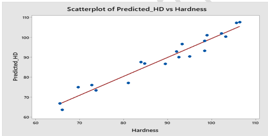
Fig. 1: Scatter plot of Predicted Hardness vs. Actual Hardness of Developed Powdered Pentaclethra Macrophylla Pod /Bio-Epoxy Resin Based Brake Pad Composite.
