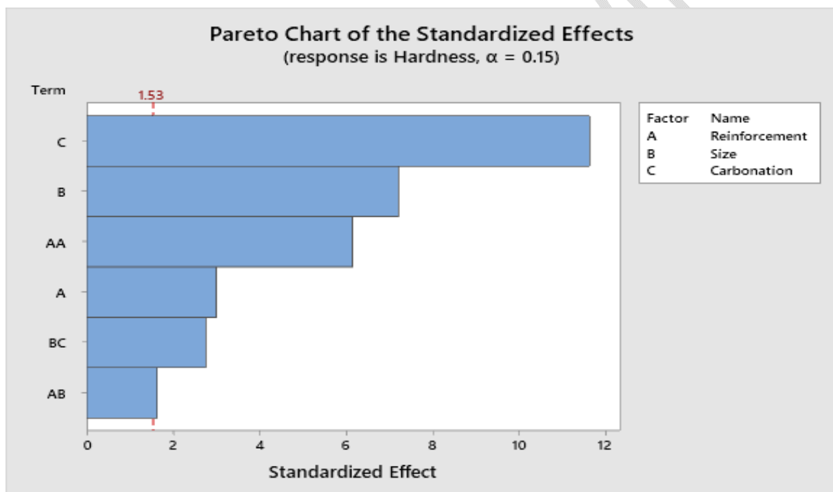
Fig. 2: Pareto Chart for Hardness of Developed Powdered Pentaclethra Macrophylla Pod /Bio-Epoxy Resin Based Brake Pad Composite.
