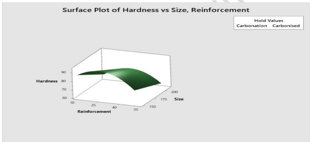
Fig. 4a: Surface Plot (3-D) for Hardness of Developed Carbonized Powdered Pentaclethra Macrophylla Pod /Bio-Epoxy Resin Based Brake Pad Composite.
