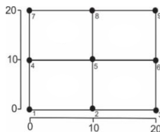
Figure 1. Erosion Plot Measuring 20 m x 20 m.
