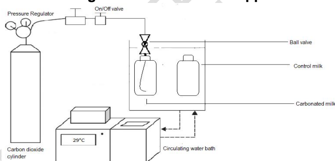
Figure 01. Carbonation Apparatus
