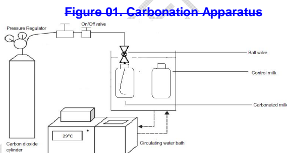
Figure 01. Carbonation Apparatus
