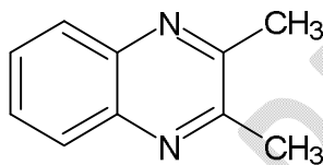
Fig 1: 2,3-dimethylquinoxaline
