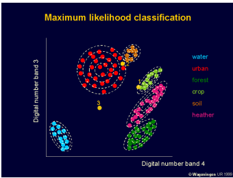
Figure2: maximum likelihood classification [14]
