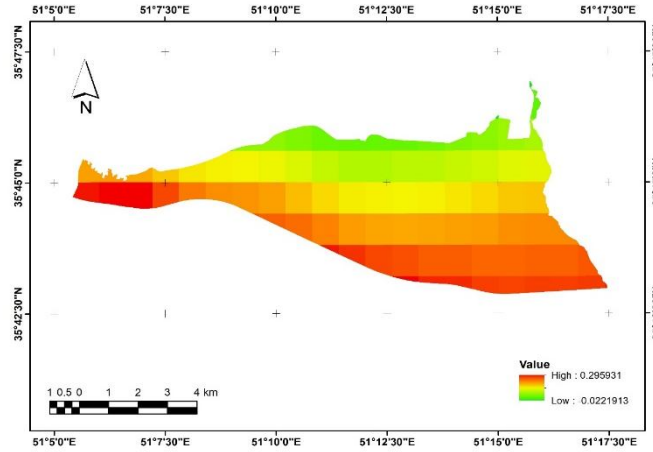
Figure 5: AI index spatial changes
