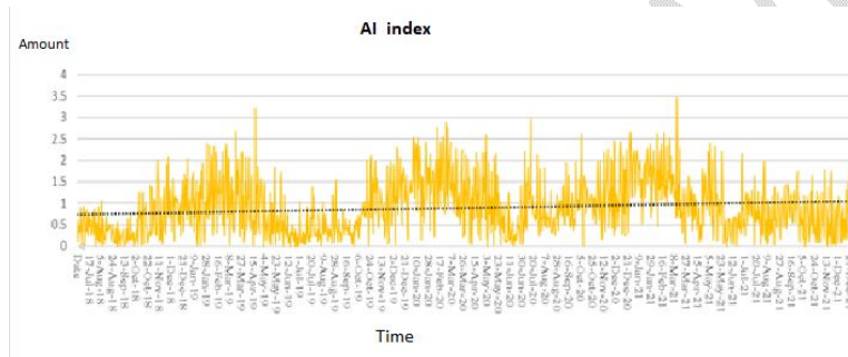
Figure 6: The trend of changes in the AI index per unit of time
