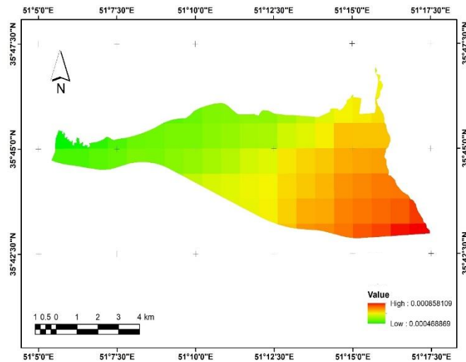
Figure 9: NO2 index spatial changes map
