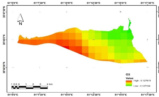
Figure 13: O3 index spatial changes map
