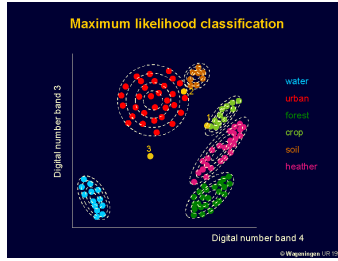
Figure2: maximum likelihood classification[14]
