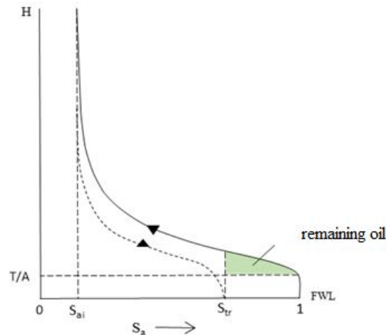
Fig.6 Capillary pressure difference curves ( s_a is saturation of water, s_{tr} is saturation in remaining oil) [5]
