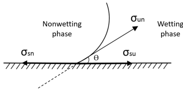
Fig.2. The contact angle of the oil to solid area [3]
