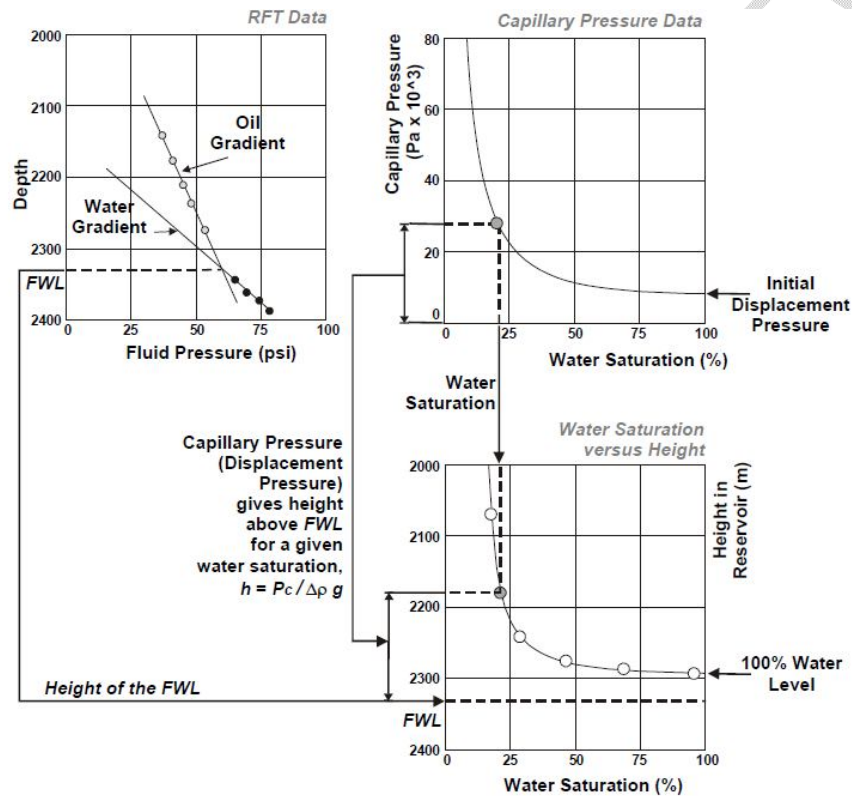
Fig.5 Method for obtaining the saturation-height function above the FWL [4].
