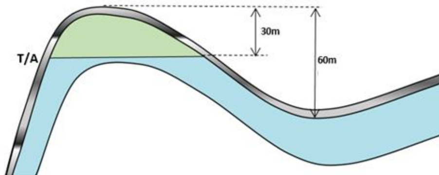
Fig.9 Oil column and reservoir closure in section
