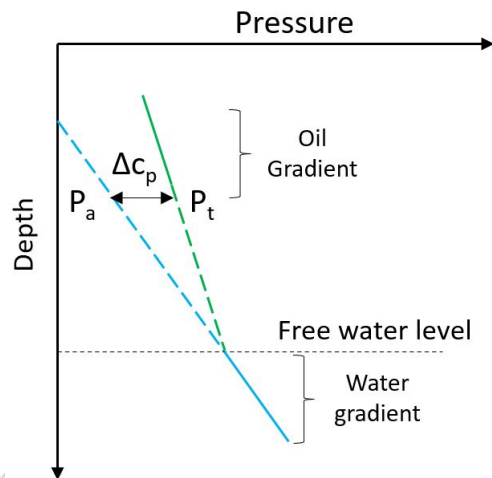
Fig.4 Plot of intersection of fluid gradients [3].
