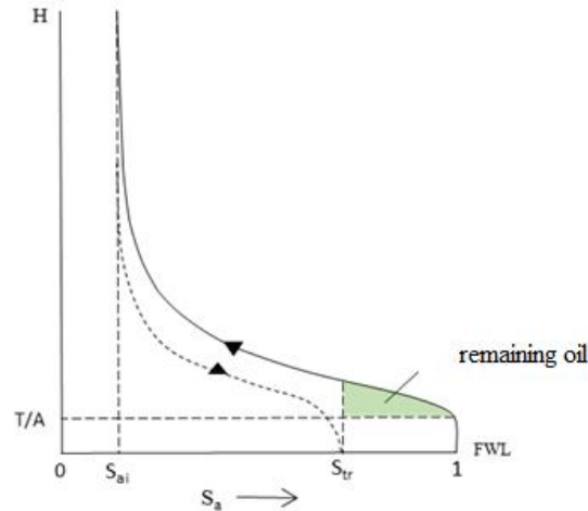
Fig.6 Capillary pressure difference curves ( s_a is saturation of water, s_{tr} is saturation in remaining oil)
