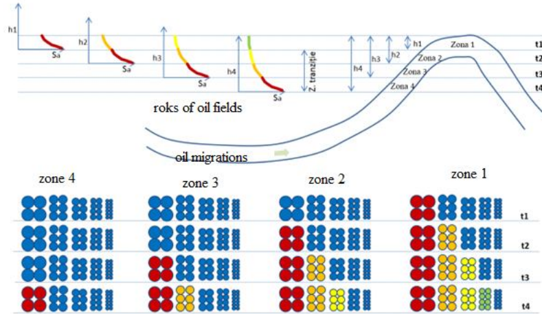
Fig.3 The crude oil migrated
