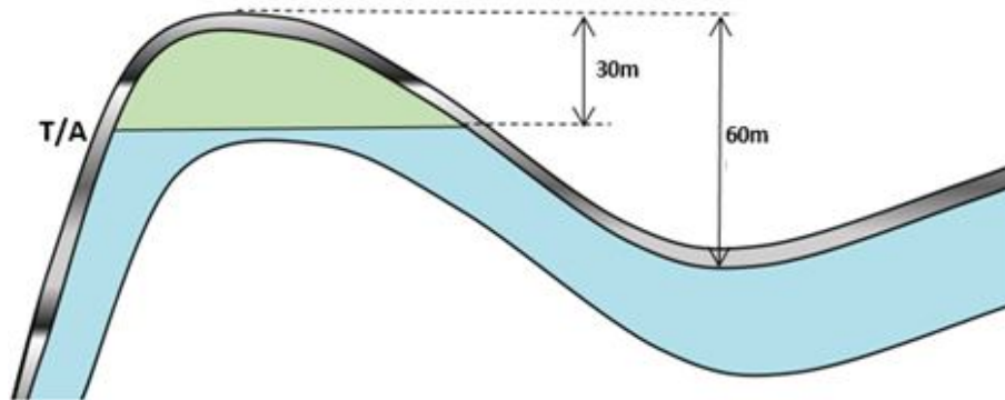
Fig.9 Crude oil column and reservoir closure in section
