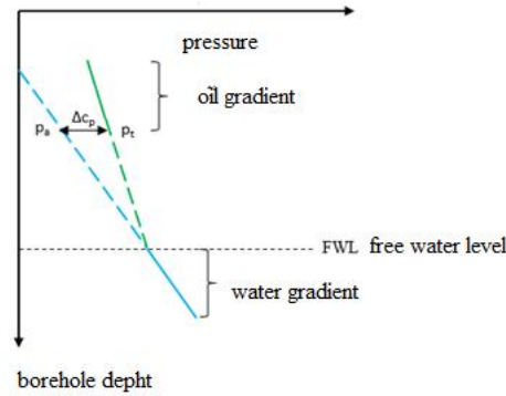
Fig.4 Plot of intersection of fluid gradients
