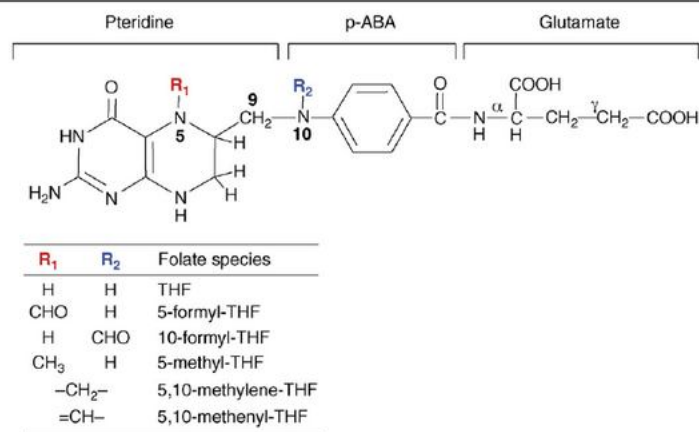
Fig.5 Molecular structure of folate showing the binding sites 22
