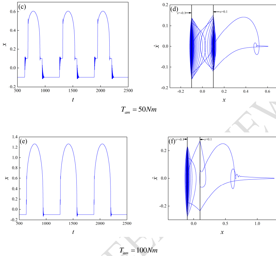
Fig. 5 The dynamical oscillations of the system when there are different external excitation responses.
