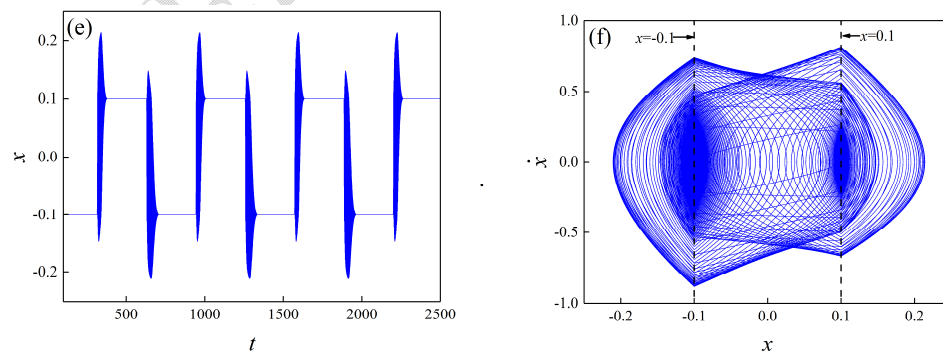
Fig. 4 The dynamical oscillations of the system when there are different torsional stiffness coefficients.
