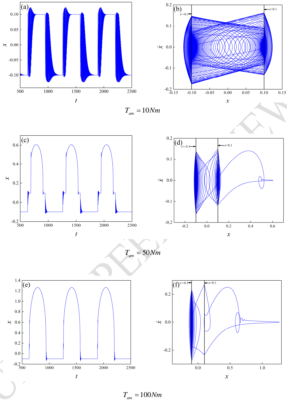
Fig. 5 The dynamical oscillations of the system when there are different external excitation responses.
