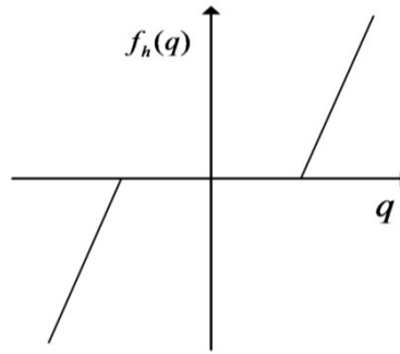
Fig. 1 Non-linear segmented functions of the gear gap clearance f_h(q) .
