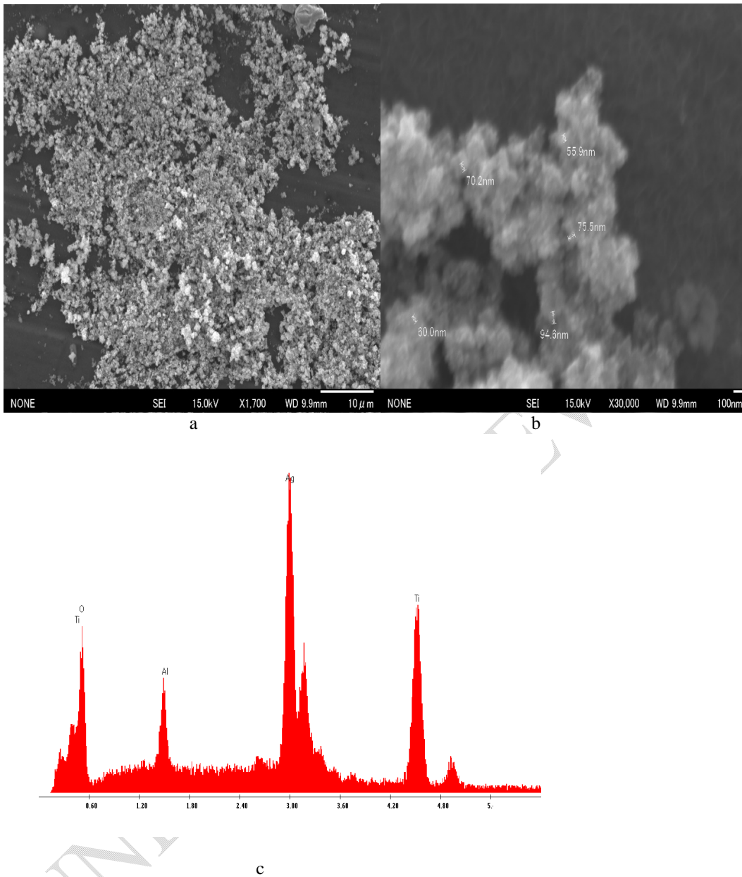
Fig. 2. (a)(b) SEM image of the Al surface functionalized with APTMS at pH 3 adjusted using dilute \text{HNO}_3 ; (c) point EDS pattern of the Al surface
