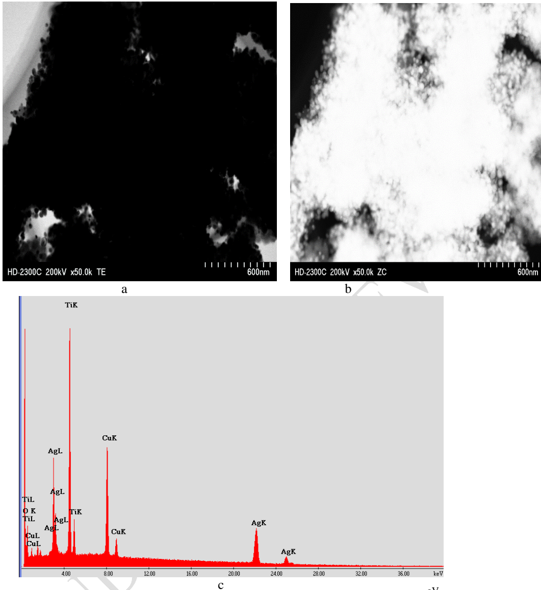
Fig. 1. (a) TEM images of an anatase ( \text{TiO}_2 ) surface coated using Ag at pH 3, (b) high-angle annular dark-field image of Ag- \text{TiO}_2 , (c) point EDS pattern of the \text{TiO}_2 surface. The copper signal is from the TEM sample grid.
