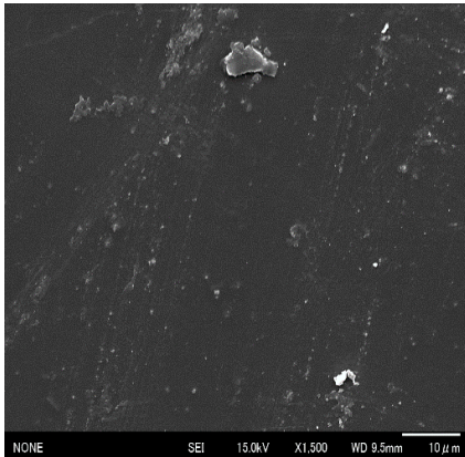
Fig. 7. (a) SEM image of the glass surface at pH 2 adjusted using dilute \text{HNO}_3 , which coated by \text{Ag-TiO}_2 solution including copper ion; (b) point EDS pattern of the glass surface; (c) SEM image of the glass surface at pH 2 adjusted using dilute \text{HNO}_3 , which coated by \text{Ag-TiO}_2 solution without copper ion.
