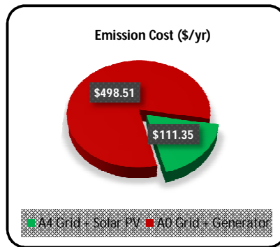
Fig. 33. Emission cost for Grid + Generator | Grid + Solar PV
