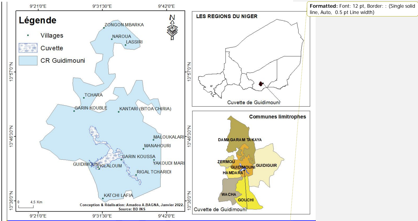
Fig.1: Location map of the study area
