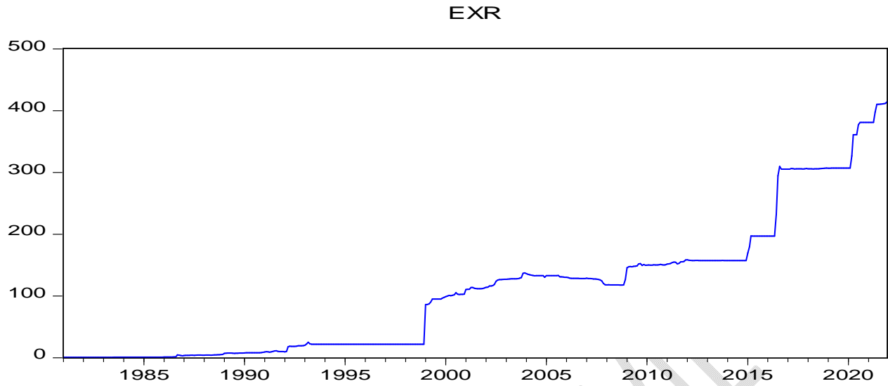
Fig. 1: Time Plot of Monthly Average Official Exchange Rate (Naira/USD) at Level D(\text{EXR})
