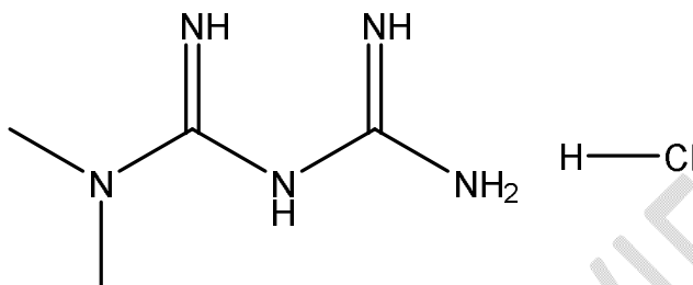
Fig. 1. Structure of metformin hydrochloride
