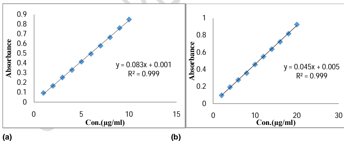
Fig.5. Standard calibration curve (a) Metformin Hydrochloride (b) Pravastatin Sodium
