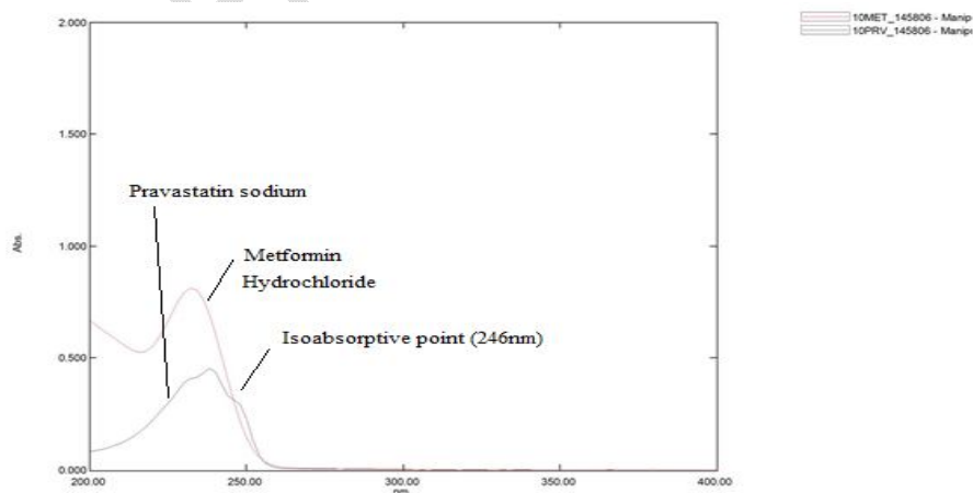
Fig. 4. Overlay spectra of Metformin Hydrochloride and Pravastatin sodium
