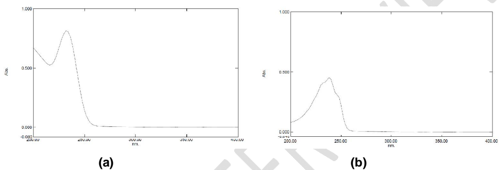
Fig.3. UV absorption spectra of Metformin Hydrochloride and Pravastatin Sodium
