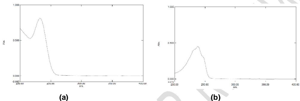
Fig. 3. UV absorption spectra of Metformin Hydrochloride and Pravastatin Sodium
