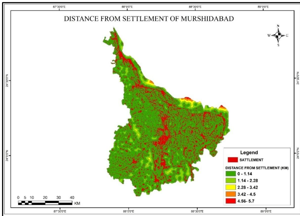
Fig. – 13 Distances from Settlement of the Study Area
