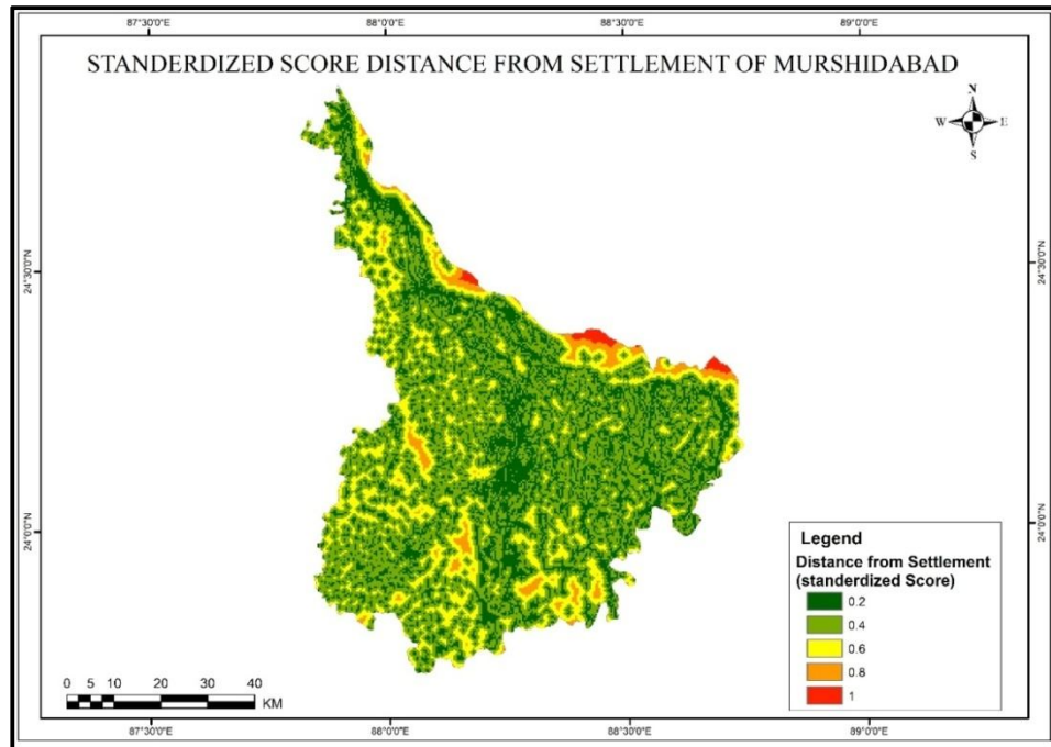
Fig. – 14 Standardized Score of Distances from Settlement
