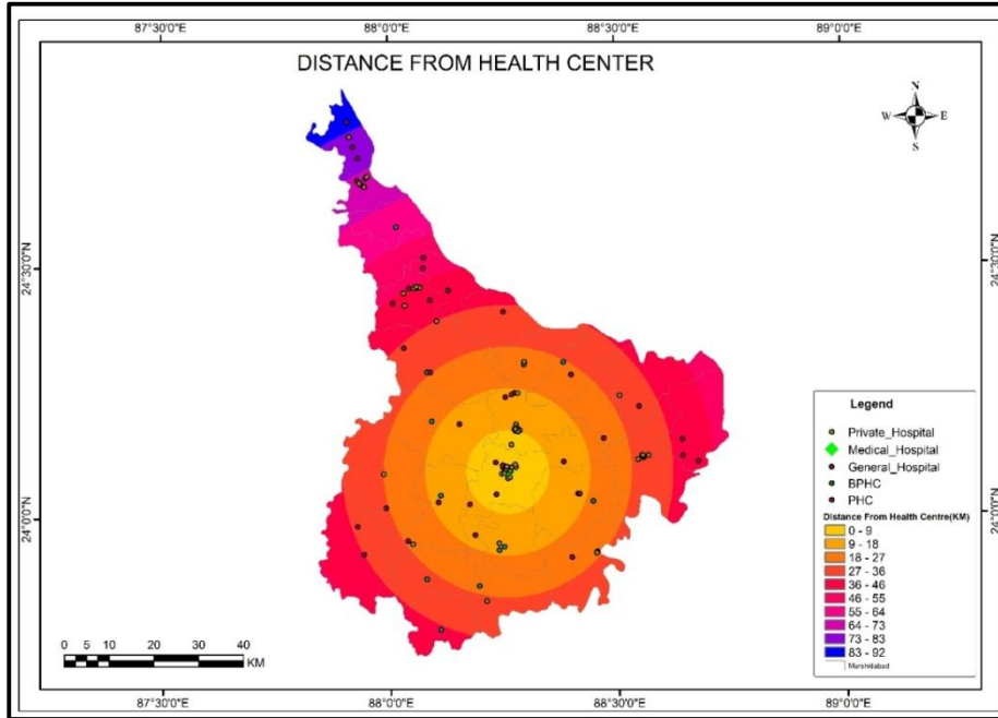
Fig. - 4 Distances from Health Center of Study Area
