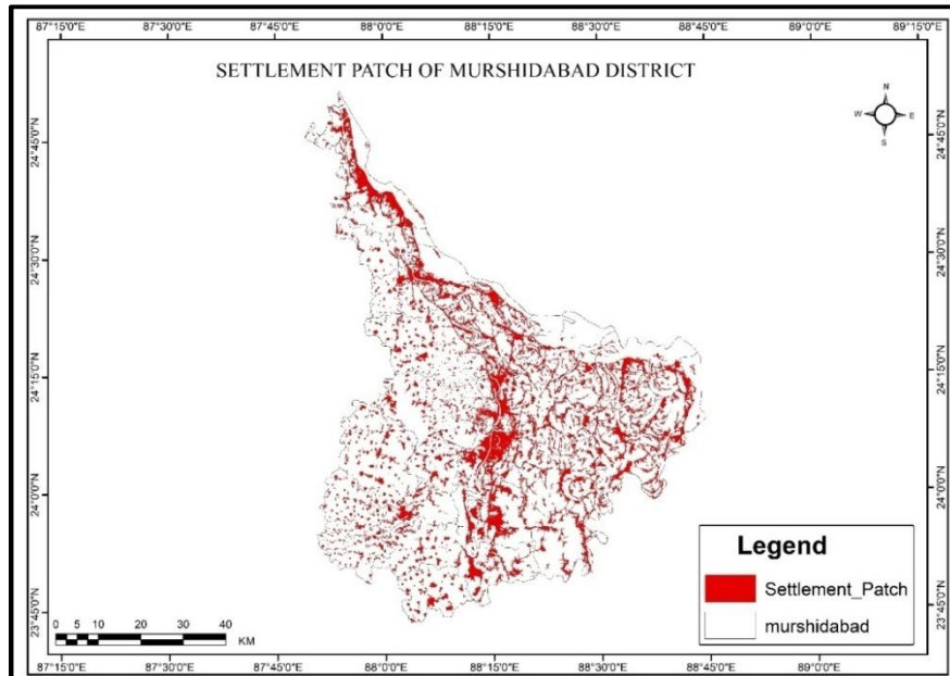
Fig. – 12 Settlement patch of the Study Area
