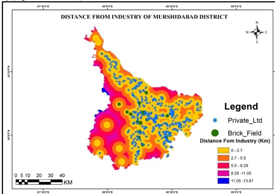
Fig. – 10 Distances from Industry of the Study Area
