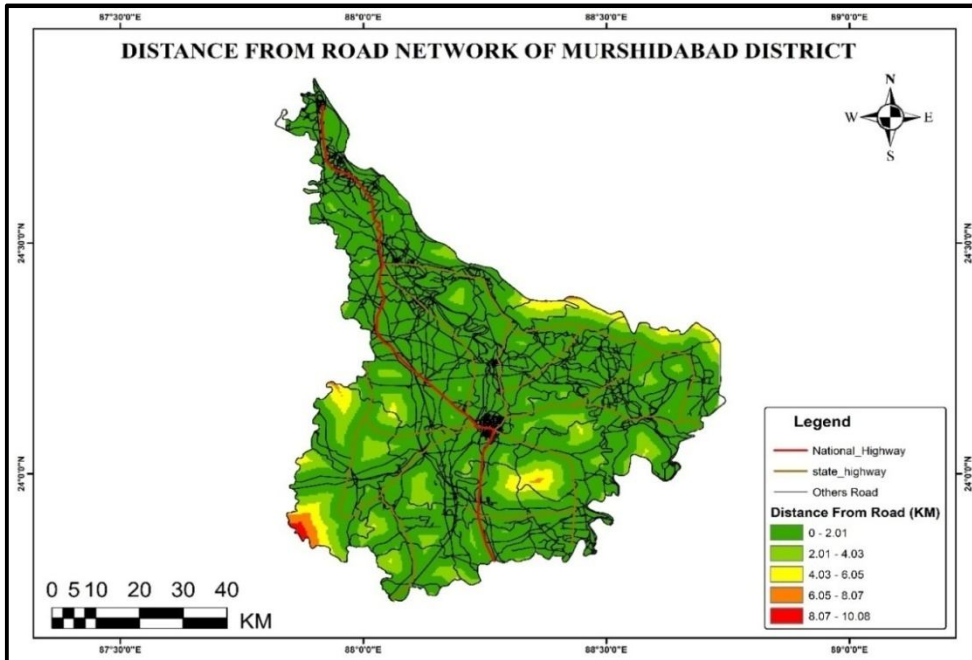
Fig. – 6 Distances from Road Network of Study Area
