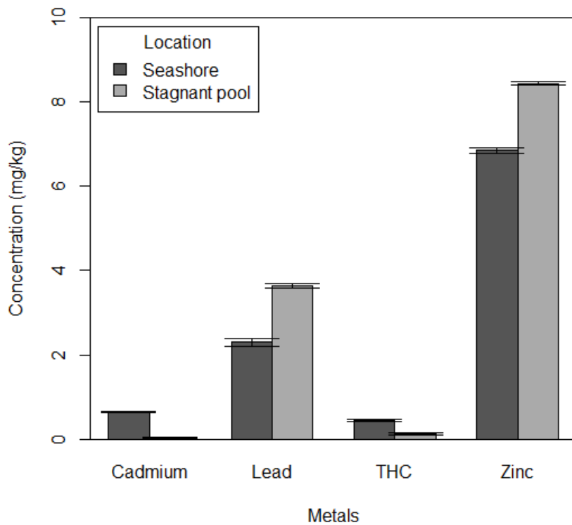
Figure 5. Physico-chemical analysis of soil at some locations at Eagle Island, Niger Delta, Nigeria. It shows that seashore has more Cd and THC while the stagnant pool has more concentration of Pb, and Zn.
