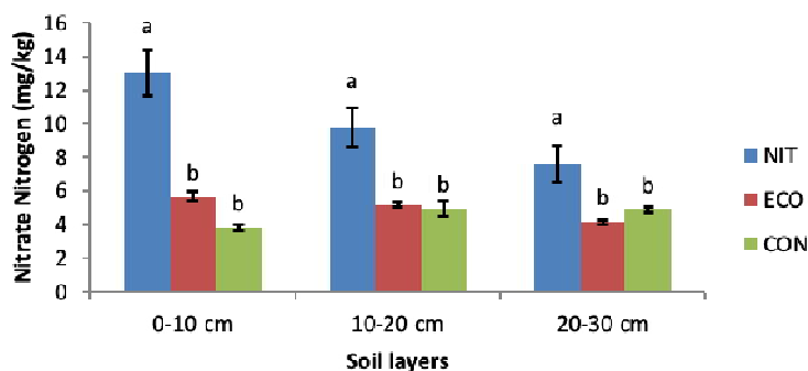
Figure 5 Effect of NIT, ECO) and CON at 0-10 cm, 10-20 cm and 20-30 cm soil levels on soil available nitrogen in mg/kg. Error bars indicate standard error. Means followed by different letters differ significantly between each tillage systems at each soil layer.
