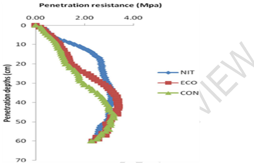
Figure 3 Effects of tillage systems on penetration resistance throughout the 0-60 cm soil profile. Average values for 10 samplings per 6 replicates are presented.
