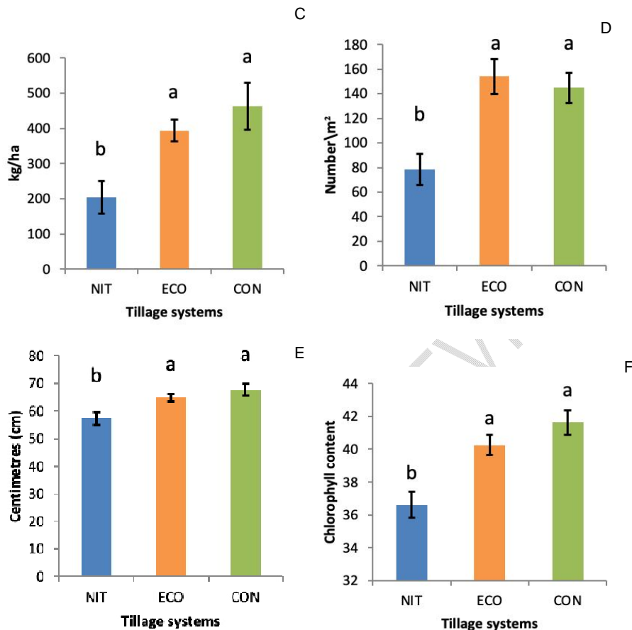
Figure 8 Effect of tillage systems on crop performance (A, B, C, D, E and F for LAI, Total DM, ear DM, Ear/m 2 , height and SPAD respectively). Error bars indicate standard error. Means followed by different letters differ significantly between each tillage systems.
