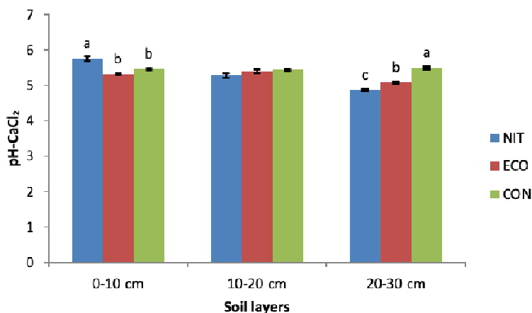
Figure 7 Effects of NIT, ECO and CON at 0-10 cm, 10-20 cm and 20-30 cm soil levels on soil pH-CaCl 2 . Error bars indicate standard error. Means followed by different letters differ significantly between each tillage systems at each soil layer.
