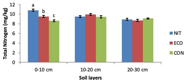
Figure 6 Effects of NIT, ECO and CON at 0-10 cm, 10-20 cm and 20-30 cm soil levels on total nitrogen in mg/kg. Error bars indicate standard error. Means followed by different letters differ significantly between each tillage systems at each soil layer.
