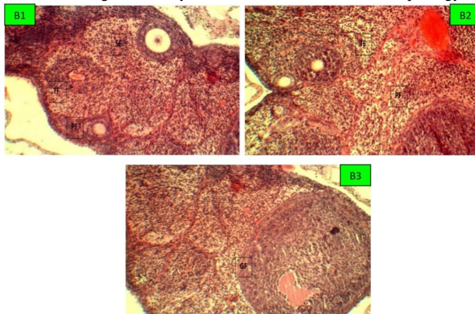
Figure 5:(B1 – B3) Photomicrograph of the ovary of female Wistar rats. B1: Group 1 (Control); B2: Group 2 animals treated with 400.0mg/kg ethanolic extract of P. yohimbestem bark; Group 3 animals treated with 800.0 mg/kg ethanolic extract of P. yohimbestem bark. Primordial follicle (PF); Secondary follicle (SF); Tertiary follicle (TF); Graafian follicle (GF);Magnification: H&E x200
