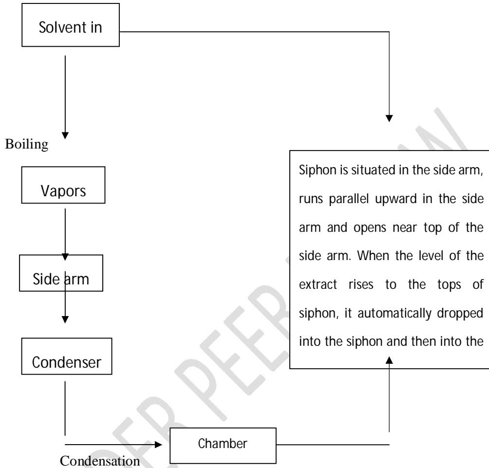
Fig. 2.2 Flow Diagram showing Extraction Process
