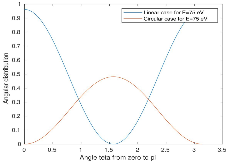
Figure 3: Curves of superposition of the angular distribution of photoelectron in the two cases of polarization h\nu = 75\text{eV}
