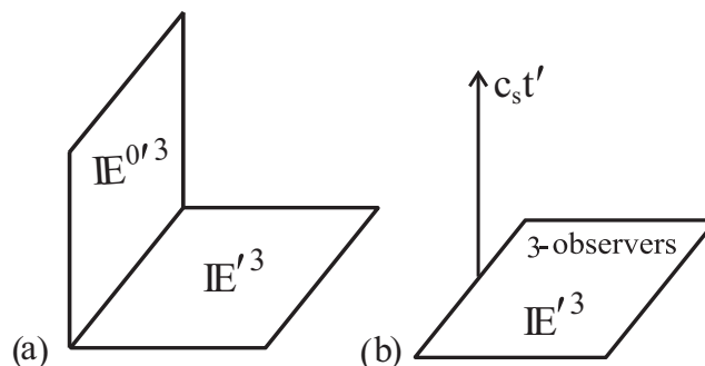
Figure 4: Figure 4a naturally transforms into Fig. 4b with respect to 3-observers in the proper Euclidean 3-space \mathbb{E}'^3 ; (Figs. 1 and 4a of [3])
