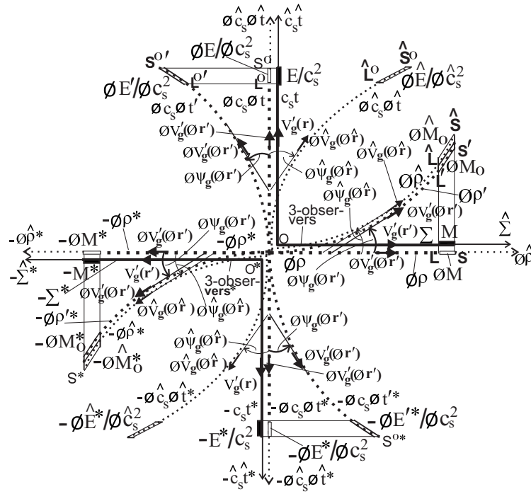
Figure 8: The global metric spacetime/intrinsic metric spacetime geometry of combined first and second stages of evolutions of spacetime/intrinsic spacetime and parameters/intrinsic parameters within the identical gravitational fields of a pair of symmetry-partner sources in the positive and negative universes, with respect to 3-observers in the Euclidean 3-spaces in the two universes, which evolves upon the geometry of Fig. 7 at the first stage.
