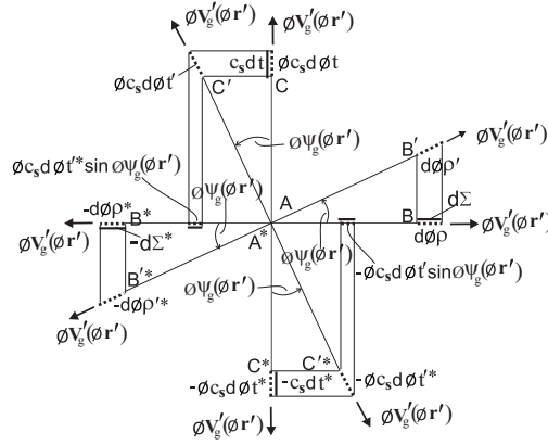
Figure 12: Local metric spacetime/intrinsic metric spacetime diagram derived from the global diagram of Fig. 8 is valid respect to 3-observers in the relativistic Euclidean 3-spaces in the positive and negative universes.
