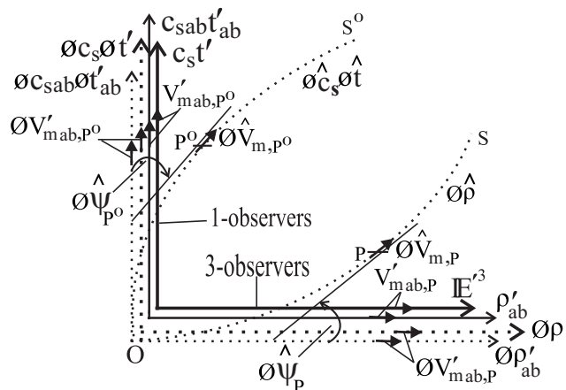
Figure 2: The flat four-dimensional relative proper metric spacetime/flat ‘two-dimensional’ absolute proper metric spacetime and hierarchy of two-dimensional intrinsic metric spacetimes that evolve at the first stage of evolutions of metric spacetimes and hierarchy intrinsic spacetimes in long-range metric force fields in our universe; (Fig. 11 of [7]).
