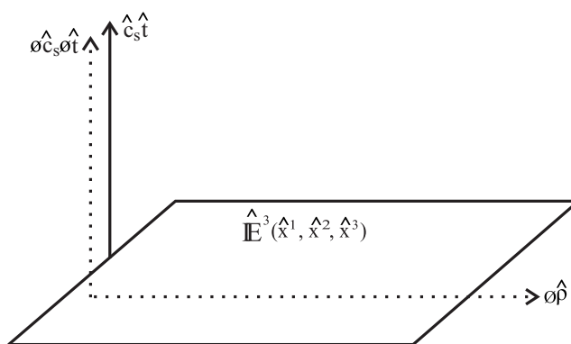
Figure 1: Flat ‘four-dimensional’ absolute metric spacetime and its underlying flat ‘two-dimensional’ absolute intrinsic metric spacetime with the assumed absence of a long-range metric force field (or absence of absolute intrinsic Riemannian spacetime geometry) in our universe; (Fig. 7 of [7]).
