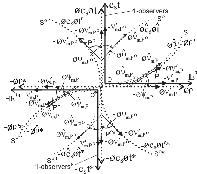
Figure 18: The inverse of the global metric spacetime/intrinsic metric spacetime diagram of Fig. 16; is valid with respect to 1-observers in the relativistic time dimensions c_s and -c_s t^* in the positive and negative universes; (Fig. 8 of [8])
