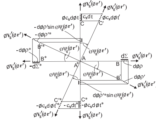
Figure 13: Local metric spacetime/intrinsic metric spacetime diagram derived from the global diagram of Fig. 9 is valid with respect to 1-observers in the relativistic metric time dimensions in the positive and negative universes; the complementary diagram to Fig. 12.
