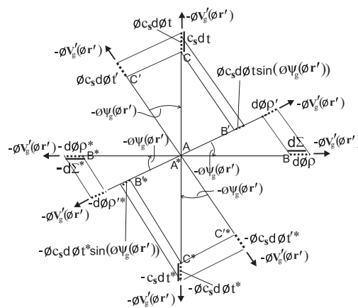
Figure 14: The inverse of Fig. 12 is valid with respect to 1-observers in the relativistic metric time dimensions in the positive and negative universes.
