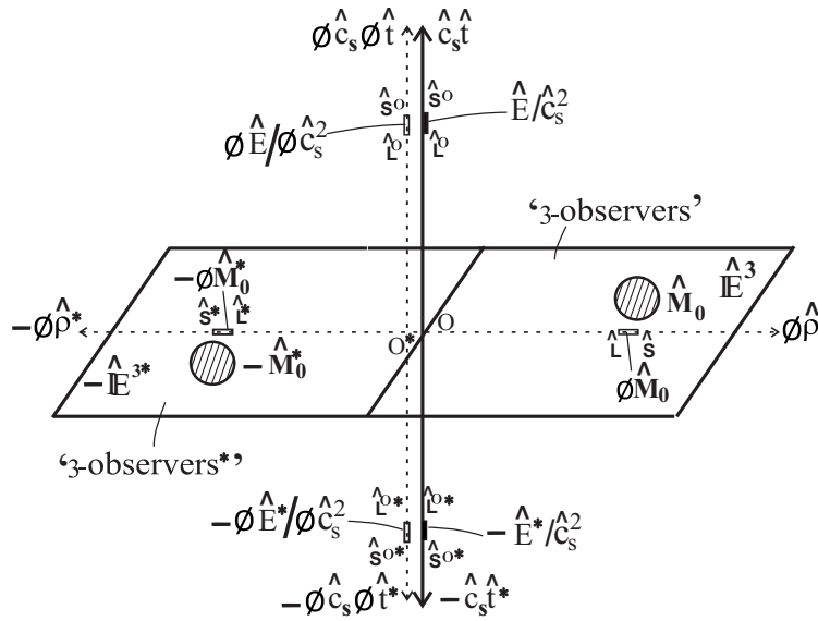
Figure 5: The diagram of Fig. 3 of four symmetrical universes in the four-world picture naturally transforms into flat ‘four-dimensional’ absolute metric spacetimes and the underlying flat ‘two-dimensional’ absolute intrinsic metric spacetimes of the positive (or our) universe and the negative universe, with respect to ‘3-observers’ in the absolute metric spaces in our universe and the negative universe.
