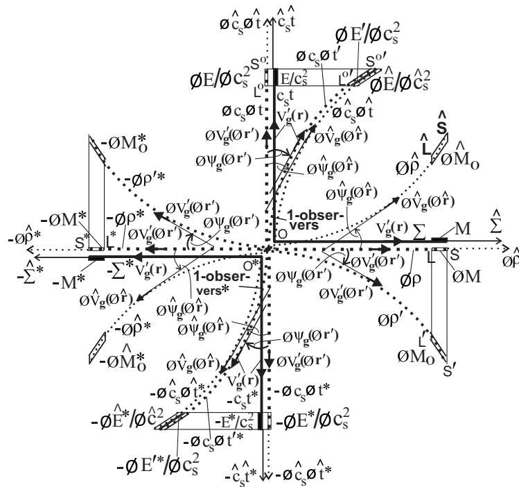
Figure 9: The complementary geometry to the global geometry of Fig. 8 is valid with respect to 1-observers in the relativistic metric time dimensions in the positive and negative universes.
