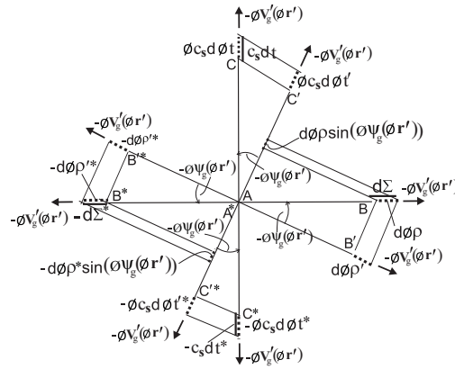
Figure 15: The inverse of Fig. 13 is valid with respect to 3-observers in the relativistic metric Euclidean 3-spaces in the positive and negative universes.
