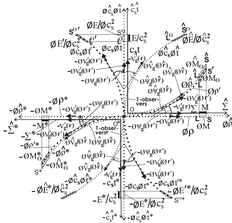
Figure 10: The inverse of the global metric spacetime/intrinsic metric spacetime geometry of Fig. 8 of combined first and second stages of evolutions of spacetimes/intrinsic spacetimes and parameters/intrinsic parameters within symmetry-partner gravitational fields in our universe and negative universe is valid with respect to 1-observers in the relativistic metric time dimensions c_s t and -c_s t^* in the two universes.
