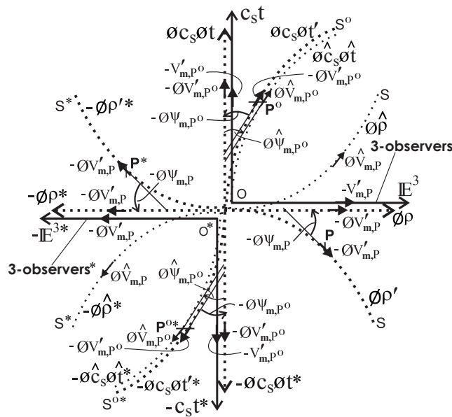
Figure 19: The inverse of the global metric spacetime/intrinsic metric spacetime diagram of Fig. 17; is valid with respect to 3-observers in the relativistic metric Euclidean 3-spaces \mathbb{E}^3 and -\mathbb{E}^{3*} of the positive and negative universes; (Fig. 9 of [8])
