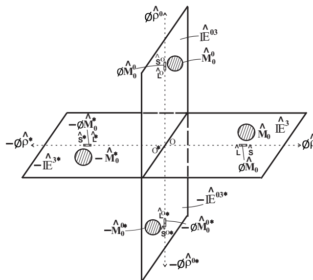
Figure 3: The mutually orthogonal flat ‘three-dimensional’ absolute metric spaces (as flat hyper-surfaces) and their underlying straight line ‘one-dimensional’ absolute intrinsic metric spaces of four symmetrical universes namely, the positive (or our) universe, the negative universe, the positive time-universe and the negative time-universe, containing identical assumed spherical absolute rest masses in the absolute metric 3-spaces and lines of absolute intrinsic rest masses in the ‘one-dimensional’ absolute intrinsic metric spaces directly underneath the absolute rest masses in the absolute spaces, of symmetry-partner gravitational field sources at symmetry-partner points in the absolute spaces within the assumed otherwise empty universes.
