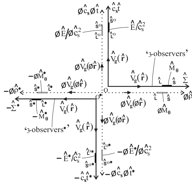
Figure 6: The absolute rest masses of symmetry-partner gravitational field sources on flat absolute metric spacetimes establish non-uniform absolute static gravitational flow speed in all their finite neighborhoods in absolute metric spacetimes and their absolute intrinsic rest masses in the underlying absolute intrinsic metric spacetimes establish non-uniform absolute intrinsic static gravitational flow speed in all their finite neighborhoods in absolute intrinsic metric spacetimes in the positive and negative universes.
