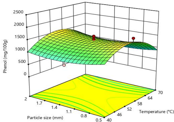
Fig.3: Effect of Temperature and Particle Size on Phenol
